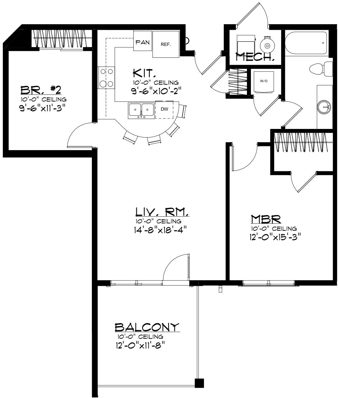
UNIT 209/308/405 FLOOR PLAN
