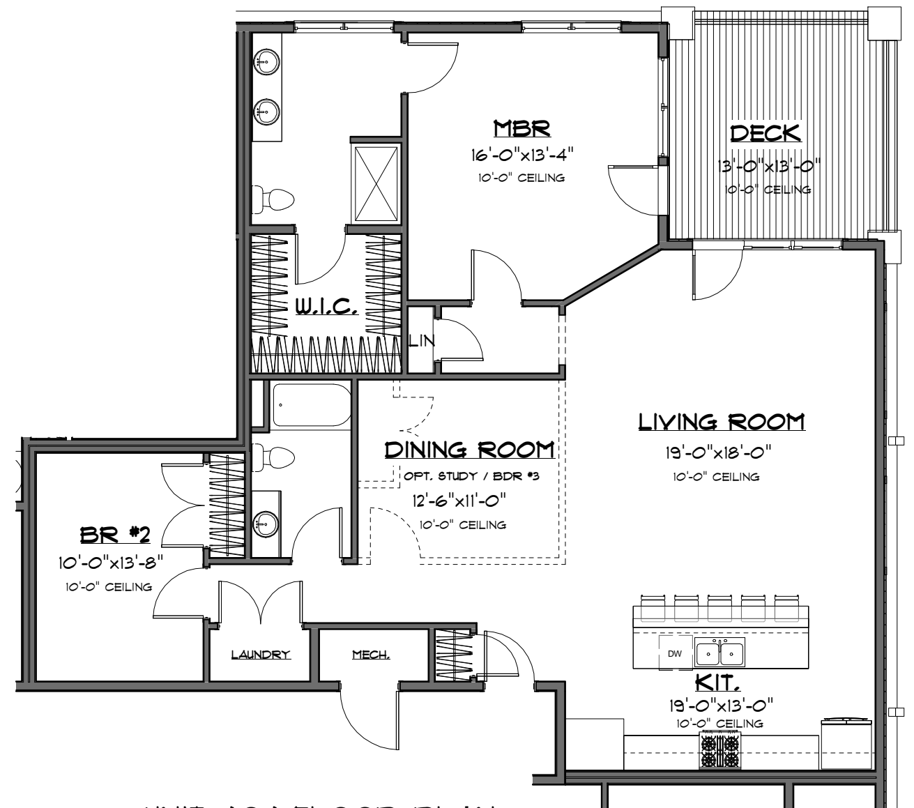
UNIT 404 FLOOR PLAN TOTAL AREA: ± 1,853 SQ. FT.
